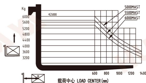
6.0T载荷曲线图 6.0T load curve
