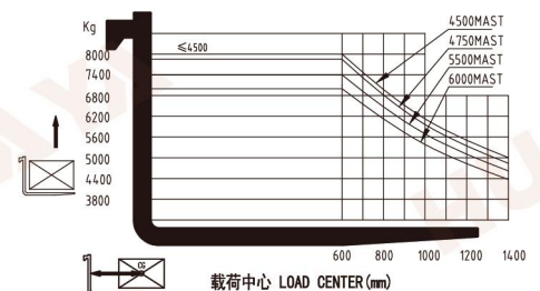
8.0T载荷曲线图 8.0T load curve
