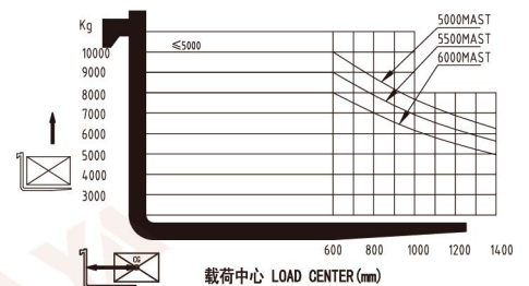
10T载荷曲线图 10T load curve
