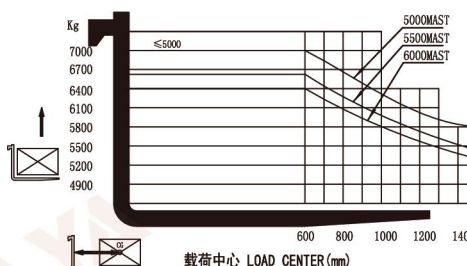
7.0T载荷曲线图 7.0T load curve
