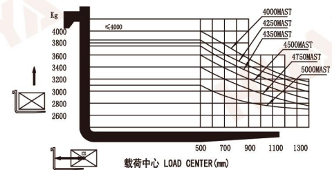
4T载荷曲线图 4T load curve
