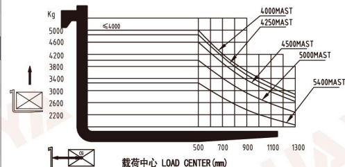
5.0T载荷曲线图 5.0T load curve
